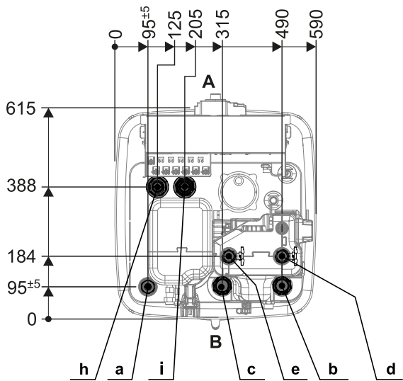
300 Litres Dimensions top-view
