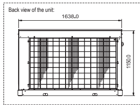
Back view of the unit
