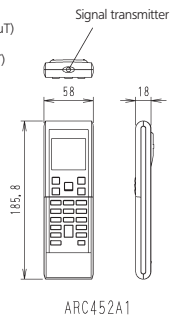
Infrared remote control
