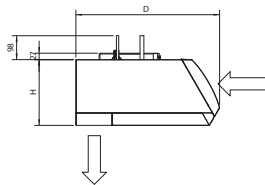
Suction grid with filter
